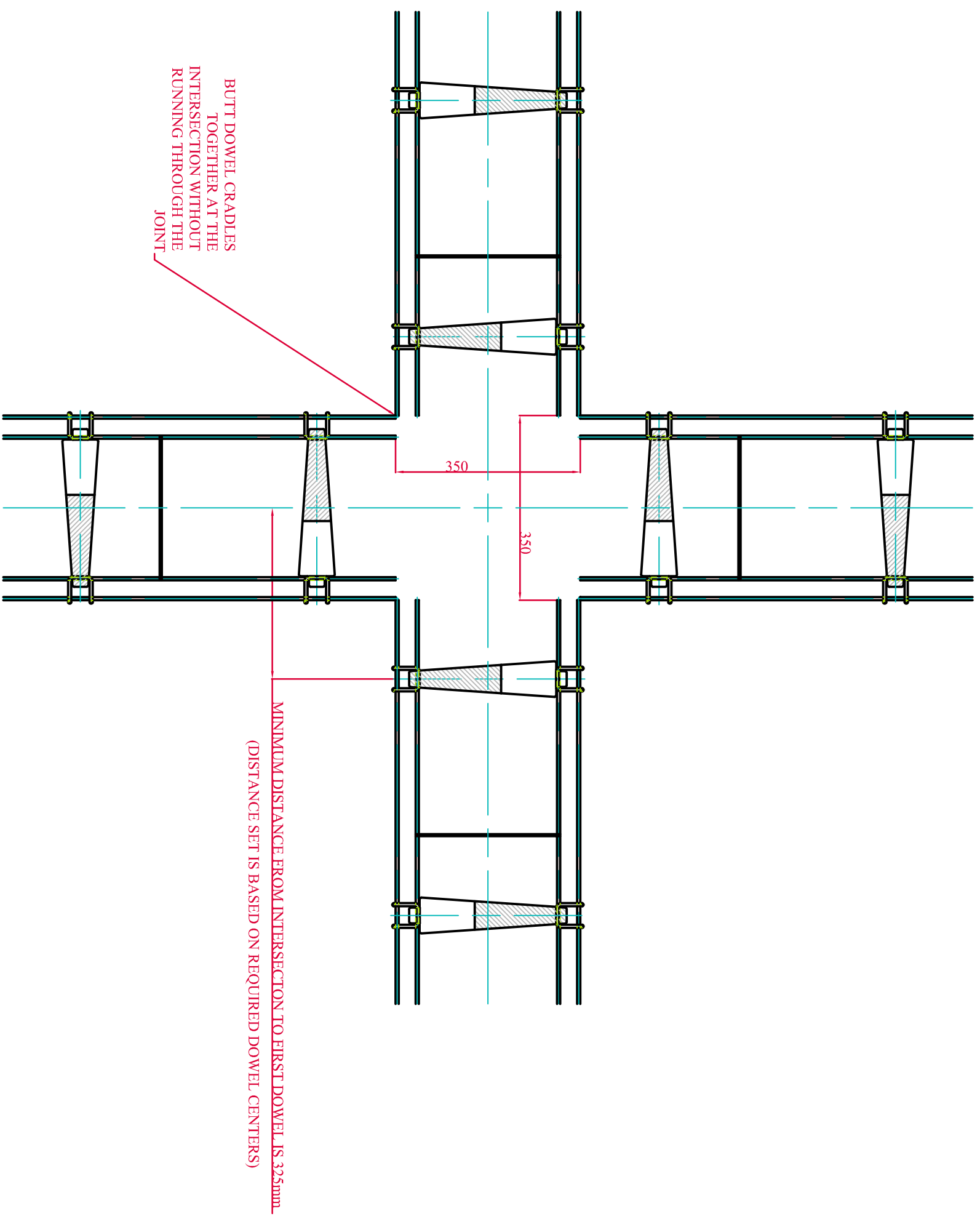
PLAN VIEW AT 4-WAY INTERSECTION
