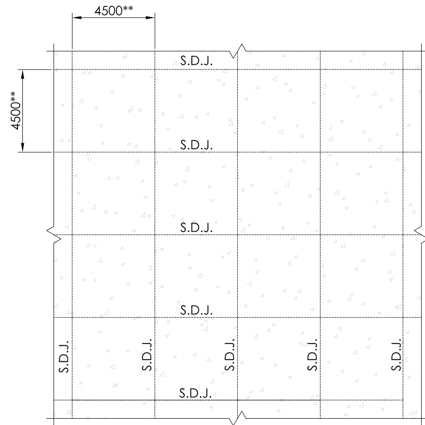
STRATEGIC REINFORCED SLAB SCALE: 1:200
