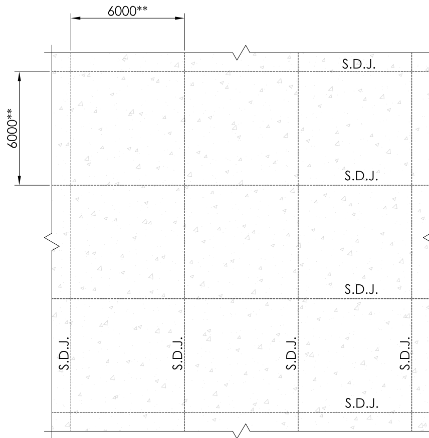
FIBRE REINFORCED SLAB SCALE: 1:200
