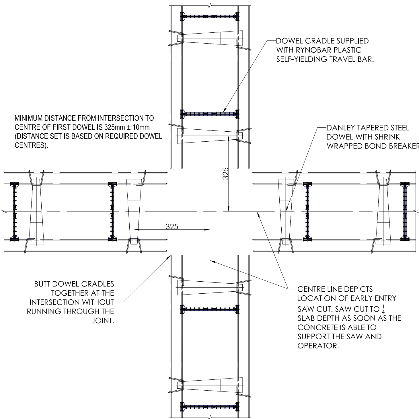
PD3 CRADLE AT 4-WAY INTERSECTION SCALE: 1:10
