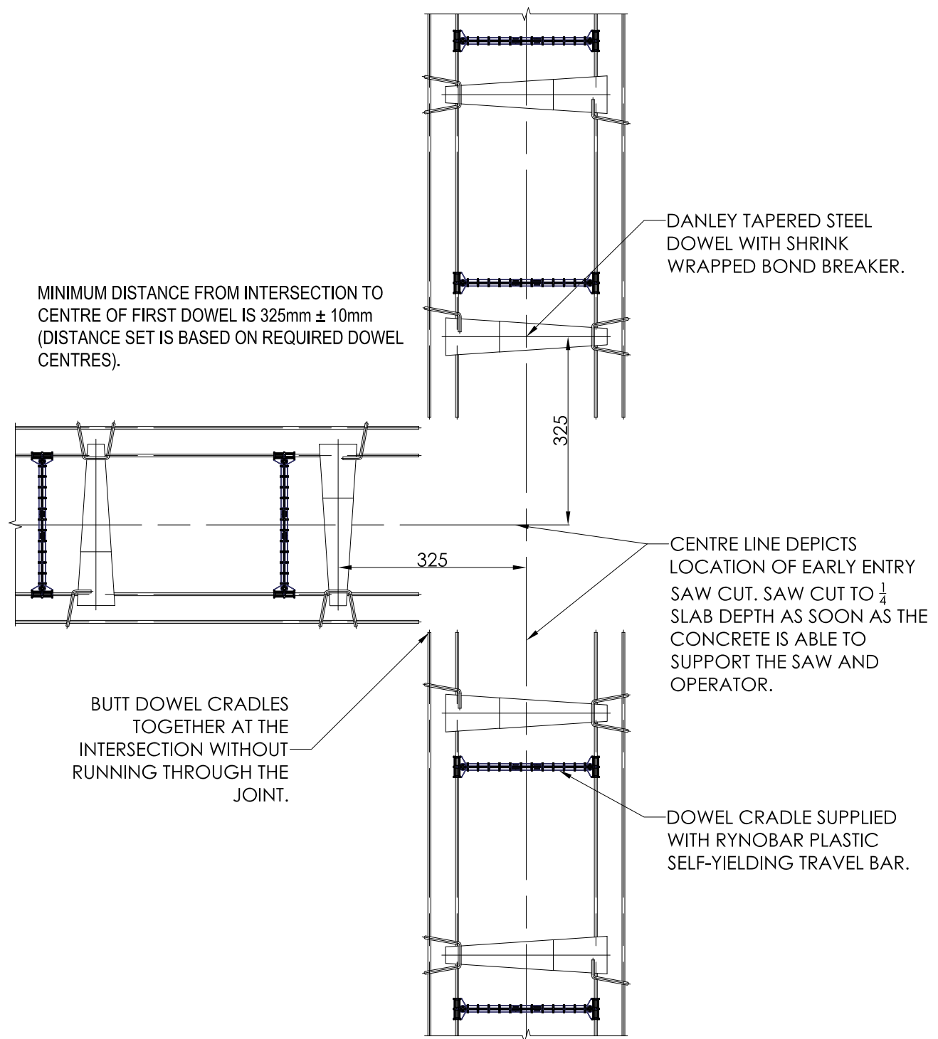
PD3 CRADLE AT 3-WAY INTERSECTION SCALE: 1:10
