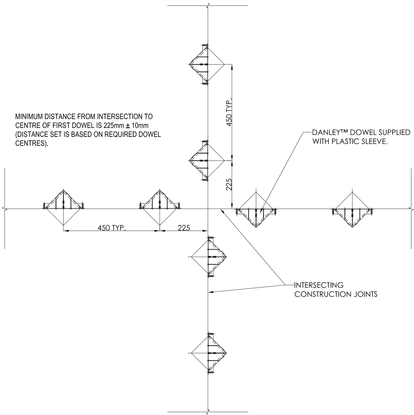
DANLEY DOWEL AT 4-WAY INTERSECTION SCALE: 1:10
