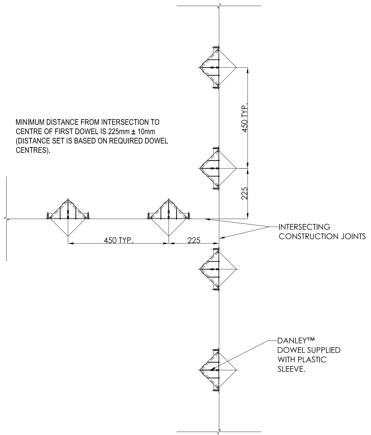
DANLEY DOWEL AT 3-WAY INTERSECTION SCALE: 1:10
